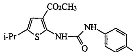
5-Isopropyl-2-(3-p-tolyl-ureido)-thiophene-3-carboxylic acid methyl ester
